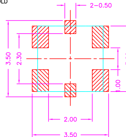
P.C.B. LAYOUT TOP VIEW ±0.05
